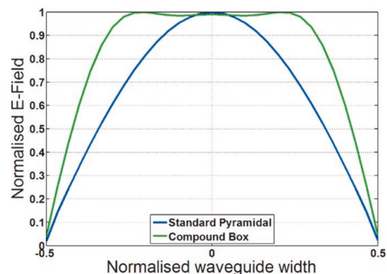
The comparative field magnitude across the waveguide section at the start of the horn flare in a pyramidal and a compound box horn.
