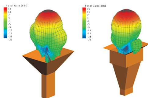
The comparative radiation patterns of a pyramidal and compound box horn with the same gain (note the smaller physical aperture size of the compound box horn.)
