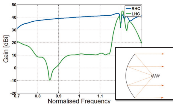
The on-axis circular polarisation performance of a typical backfire-helix-fed parabolic reflector antenna.
