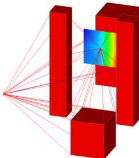
Optimising interrogator antenna placement in a warehouse or factory with UTD ray tracing.
